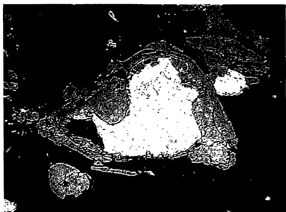
Fig. 7. Reflected light photomicrograph (50× magnification) of a sulfide rimmed metal grain from ALH-764. The triangular shaped, small dark grain at the left edge of the metal is an iron oxide. The two layer structure of the sulfide rim is clearly developed. The field of view is 0.5 mm.
