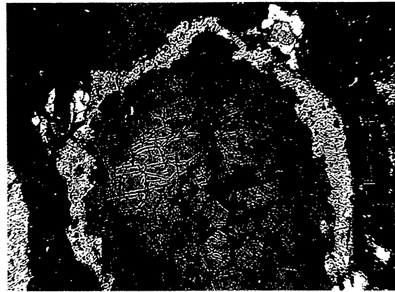
Fig. 5. Reflected light photomicrograph (12.5 \times magnification) of a silicate chondrule (from ALH-764) rimmed by metal and sulfide. The field of view is 2 mm.
