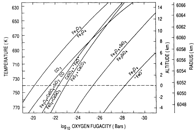
Fig. 6. The temperature-dependent oxygen fugacity (CO/CO 2 ) in the lower atmosphere of Venus is compared to the oxygen fugacities buffered by different iron-bearing mineral assemblages that may exist on the surface of Venus. Mineral assemblages to the right of the Venus atmosphere curve (CO/CO 2 ) are more reducing; those to the left are more oxidizing. As originally noted by Mueller (1964a), the oxygen fugacity at the surface of Venus is inside the magnetite (Fe 3 O 4 ) stability field. Neither wüstite (Fe 0.947 O) nor hematite (Fe 2 O 3 ) is stable under equilibrium conditions on the Venus surface. The two curves involving pyrite FeS 2 are for oxygen fugacity buffers originally proposed by Mueller (1965) for the anhydrite + wollastonite buffer and by Lewis and Kreimendahl (1980) for the anhydrite + calcite buffer. From Fegley and Treiman (1991).
