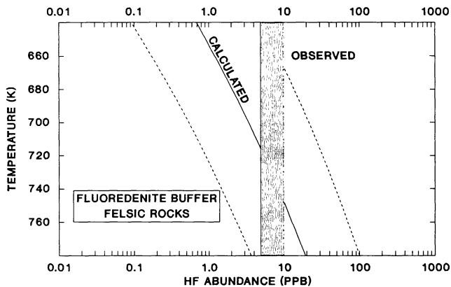
Fig. 15. A comparison of the HF abundance calculated for reaction (59) with the observed HF abundance (Bézar et al. , 1990; Connes et al. , 1967) in the atmosphere of Venus. The dashed lines indicate the range of HF values allowed by the uncertainties in the thermodynamic data. Refer to Fig. 4 to relate temperatures to altitudes on the surface of Venus. From Fegley and Treiman (1991).
