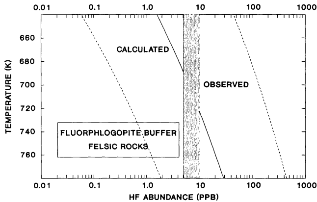
Fig. 14. A comparison of the HF abundance calculated for reaction (57) with the observed HF abundance (Bézar et al. , 1990; Connes et al. , 1967) in the atmosphere of Venus. The dashed lines indicate the range of HF values allowed by the uncertainties in the thermodynamic data. This buffering reaction was originally proposed by Lewis (1970). Refer to Fig. 4 to relate temperatures to altitudes on the surface of Venus. From Fegley and Treiman (1991).
