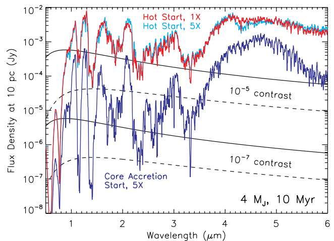
FIG. 4.—Flux density at 10 pc for 4 M_{\text{J}} objects at an age of \sim 10 Myr. In red is a hot start evolution model with solar metallicity at 1000 K. In light blue is this same model with 5\times solar metallicity, for comparison. In dark blue is a 600 K model that uses the core accretion initial condition and 5\times solar metallicity. Overplotted in black are 10^{-5} and 10^{-7} contrast ratios relative to two blackbody stars. The two solid curves are for a Sun-like 5770 K star, and the two dashed curves are for an M2 V-like 3600 K star.
