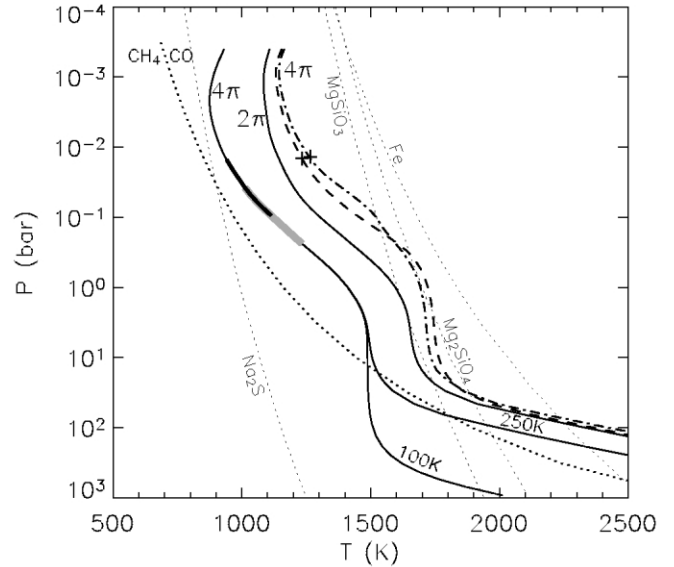
FIG. 1.—Pressure-temperature ( P - T ) profiles for TrES-1 and HD 209458b. The solid curves are two profiles for TrES-1 assuming either 2\pi (hotter) or 4\pi (cooler) reradiation of absorbed stellar flux. Both profiles assume T_{\text{int}} = 250 K. For the 4\pi case, we also plot a profile with T_{\text{int}} = 100 K. For the 4\pi profile, the thick black portion of the profile shows the extent of the brightness temperatures in the 8.0 \mu\text{m} band. The even thicker gray portion of the profile shows the brightness temperatures in the 4.5 \mu\text{m} band. We plot two 4\pi profiles for HD 209458b. The dashed curve is cloud-free, and the dash-dotted curve includes the opacity of \text{MgSiO}_3 and Fe clouds. The model brightness temperatures at 24 \mu\text{m} are marked with plus signs. The thick dotted curve is the boundary where CO and \text{CH}_4 have the same abundance. Condensation curves for \text{Na}_2\text{S} , \text{MgSiO}_3 , \text{Mg}_2\text{SiO}_4 , and Fe are thin dotted curves.
